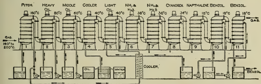
FIG. 99.—Feld System for Fractionating Coal Tar.
